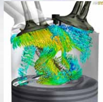
Vortex structures in a four-stroke engine just after injection of fuel and intake valve opening Courtesy of BMW Group.
