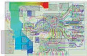
Electric potential contours on PCB trace; Joule heating of high current trace calculated as part of conjugate heat transfer solution
