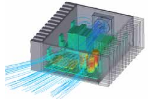
Velocity streamlines and temperature contours for fan-cooled avionics box exposed to solar radiation; model combines MCAD data and Icepak objects
