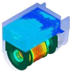
Maxwell coupled with ANSYS Fluent to determine thermal performance of induction machine
