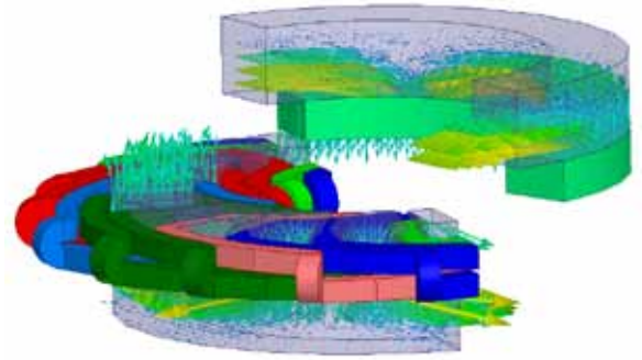
Axial magnetic field distribution on axial permanent magnet machine
