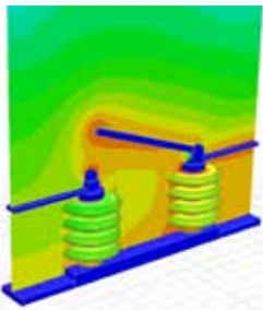
Maxwell-simulated electromagnetic field distribution on transformer terminals
